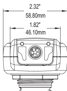
FSP-2x1B dimensions
