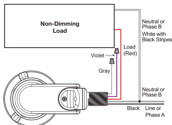
FSP-221-B wiring with non-dimming load
